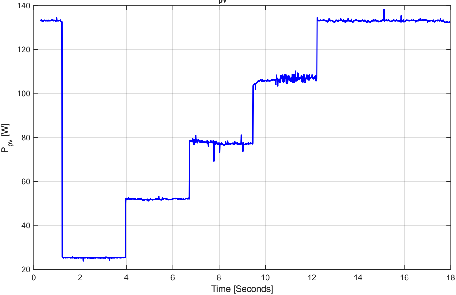
P_{pv} over Time
